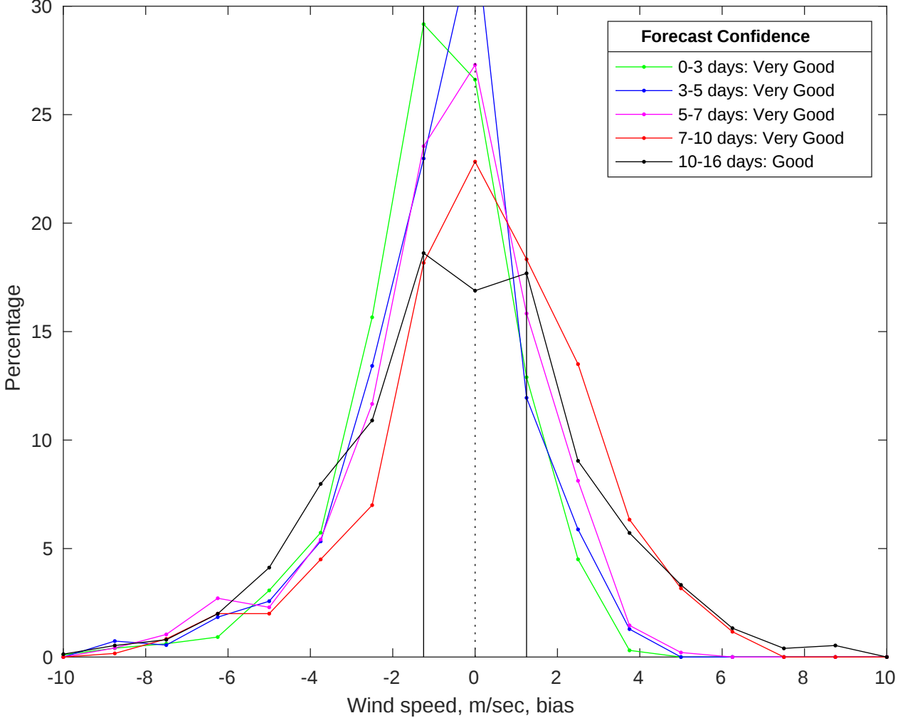
NDBC 42040 vs GFS Winds Bias Histogram: 21-Jul-2025
