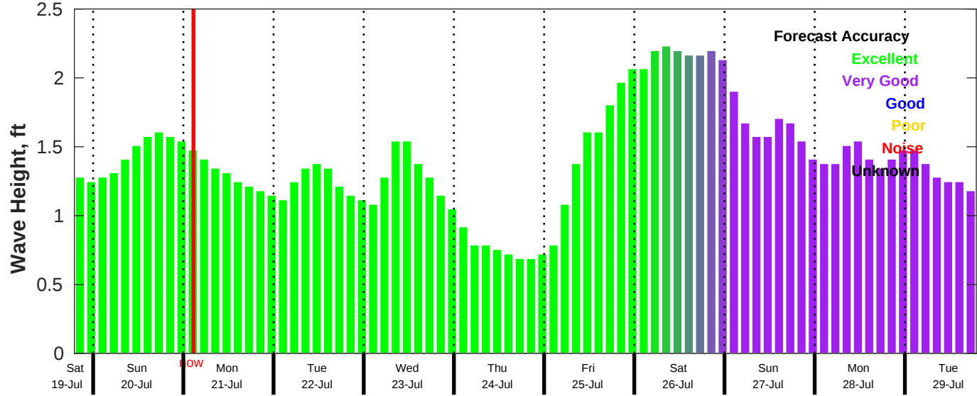
CMEMS Wave Forecast for NDBC 42040 from 19-Jul-2025 19:00:00 to 29-Jul-2025 19:00:00
