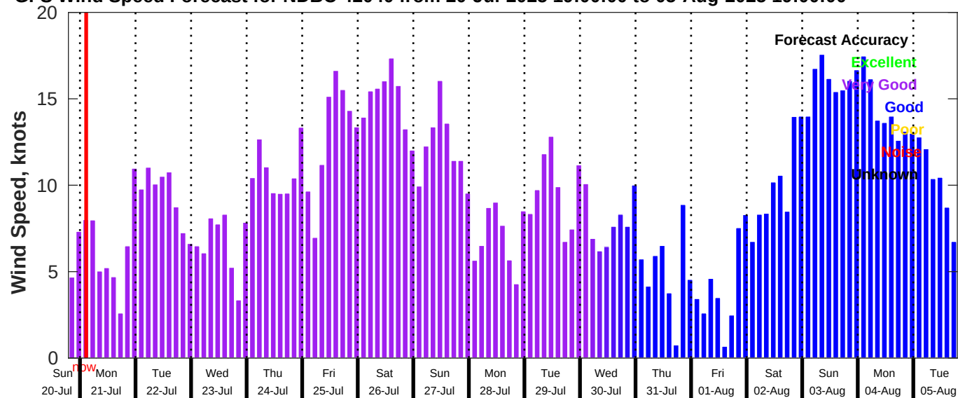
GFS Wind Speed Forecast for NDBC 42040 from 20-Jul-2025 19:00:00 to 05-Aug-2025 19:00:00
