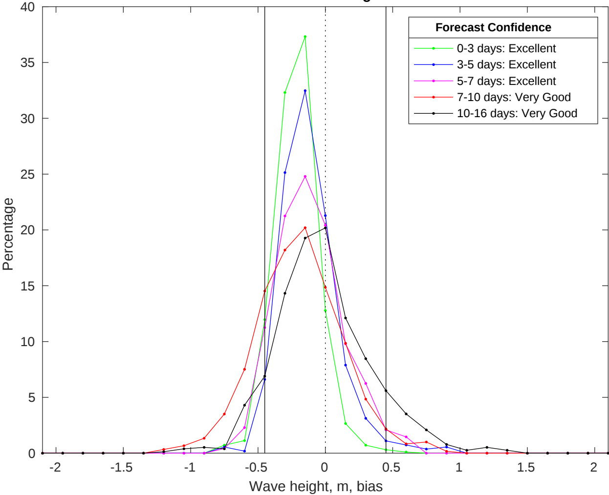
NDBC 46011 vs GFS Waves Bias Histogram: 21-Jul-2025
