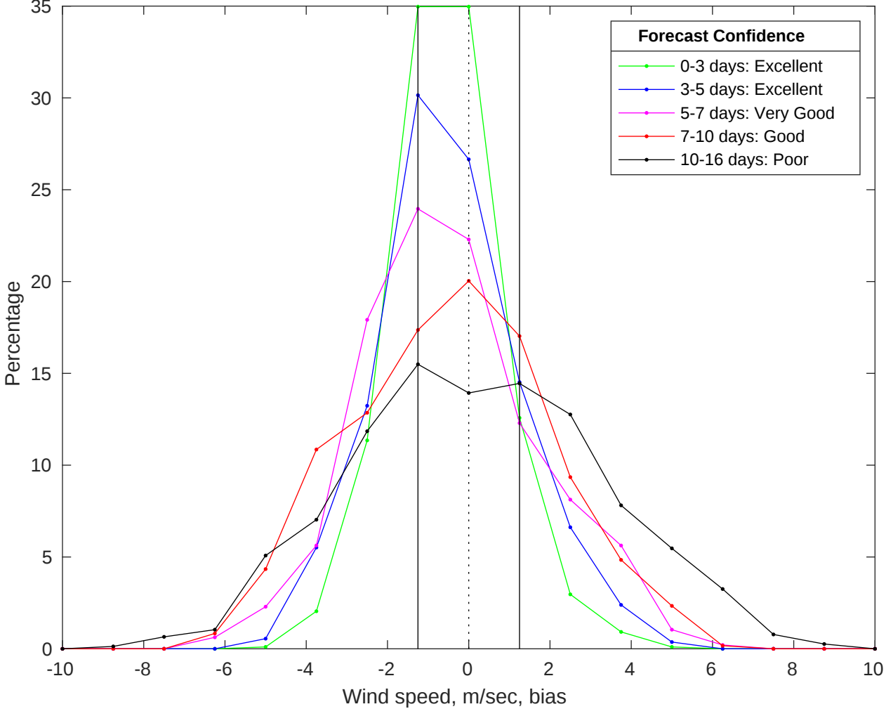
NDBC 46011 vs GFS Winds Bias Histogram: 21-Jul-2025
