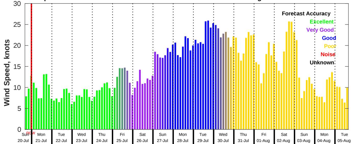
GFS Wind Speed Forecast for NDBC 46011 from 20-Jul-2025 16:00:00 to 05-Aug-2025 16:00:00
