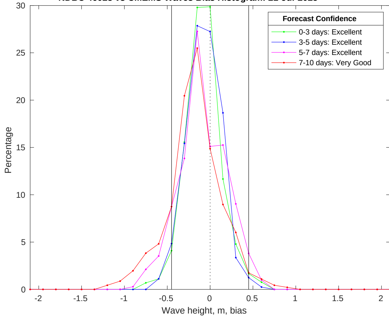
NDBC 46028 vs CMEMS Waves Bias Histogram: 21-Jul-2025
