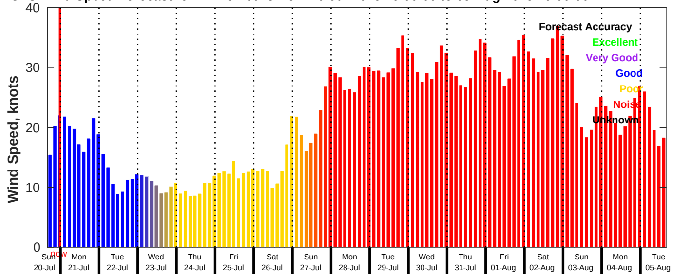
GFS Wind Speed Forecast for NDBC 46028 from 20-Jul-2025 16:00:00 to 05-Aug-2025 16:00:00
