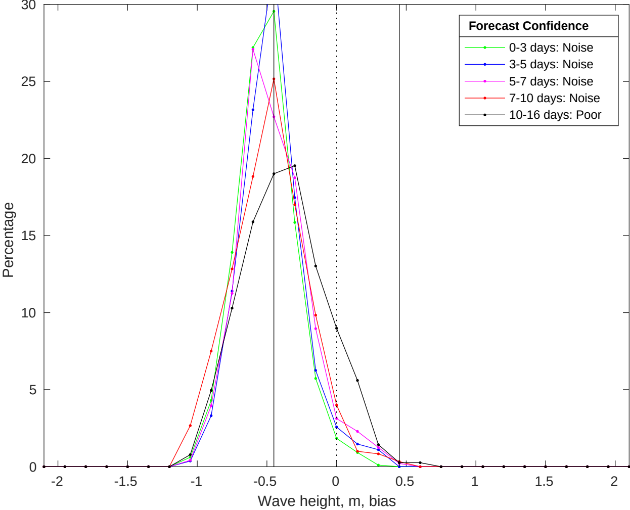
NDBC 46054 vs GFS Waves Bias Histogram: 21-Jul-2025
