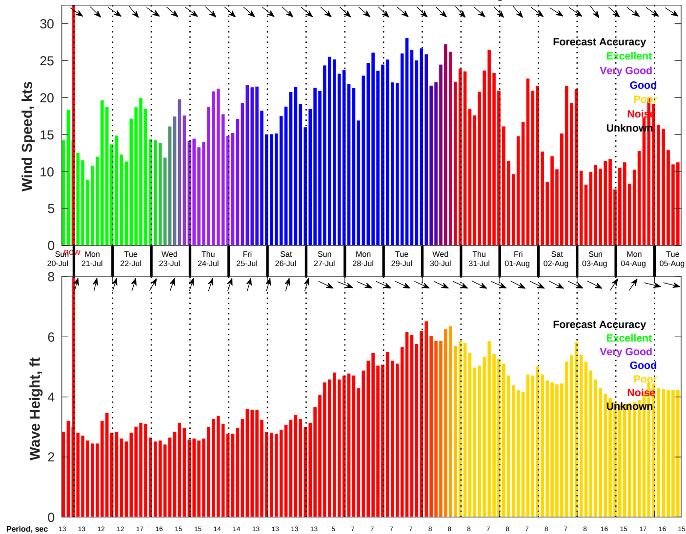
Wind & Wave Forecast for NDBC 46054 from 20-Jul-2025 16:00:00 to 05-Aug-2025 16:00:00
