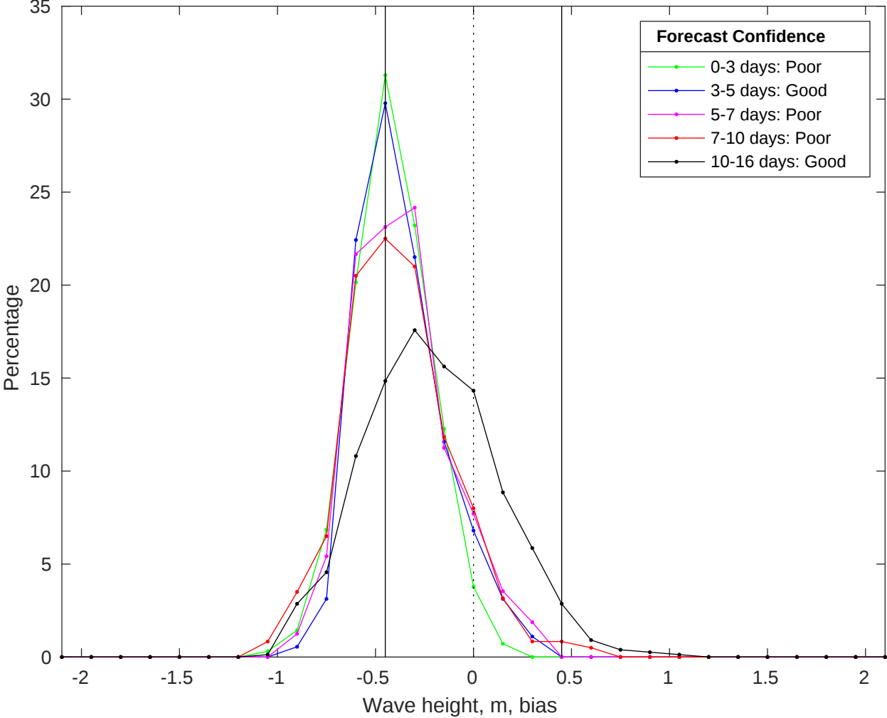
NDBC 46069 vs GFS Waves Bias Histogram: 21-Jul-2025
