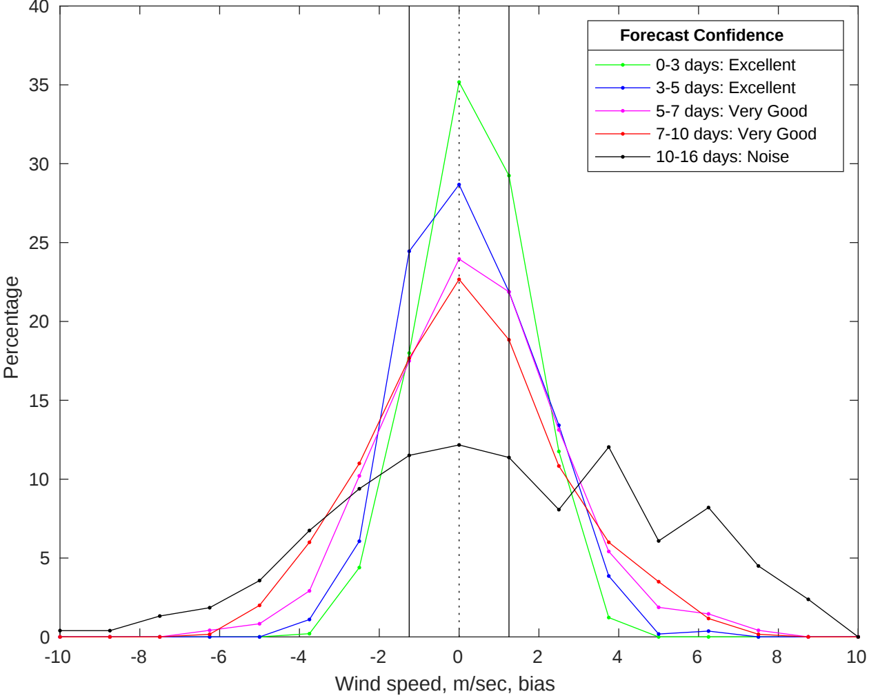
NDBC 46069 vs GFS Winds Bias Histogram: 21-Jul-2025
