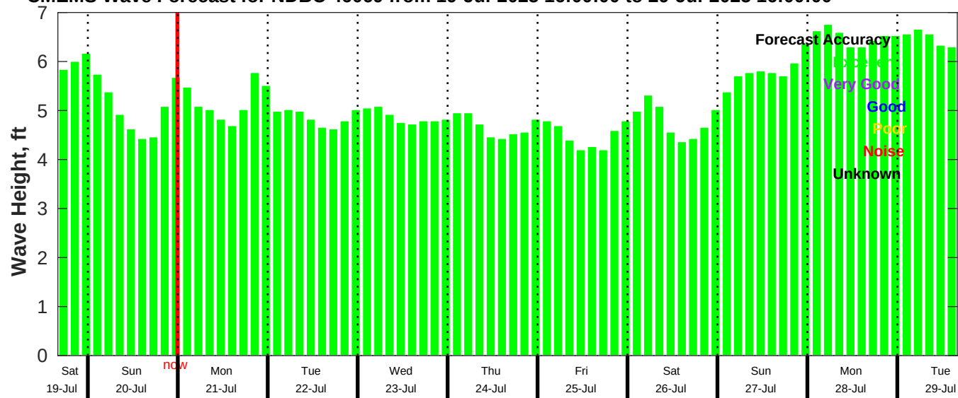
CMEMS Wave Forecast for NDBC 46069 from 19-Jul-2025 16:00:00 to 29-Jul-2025 16:00:00
