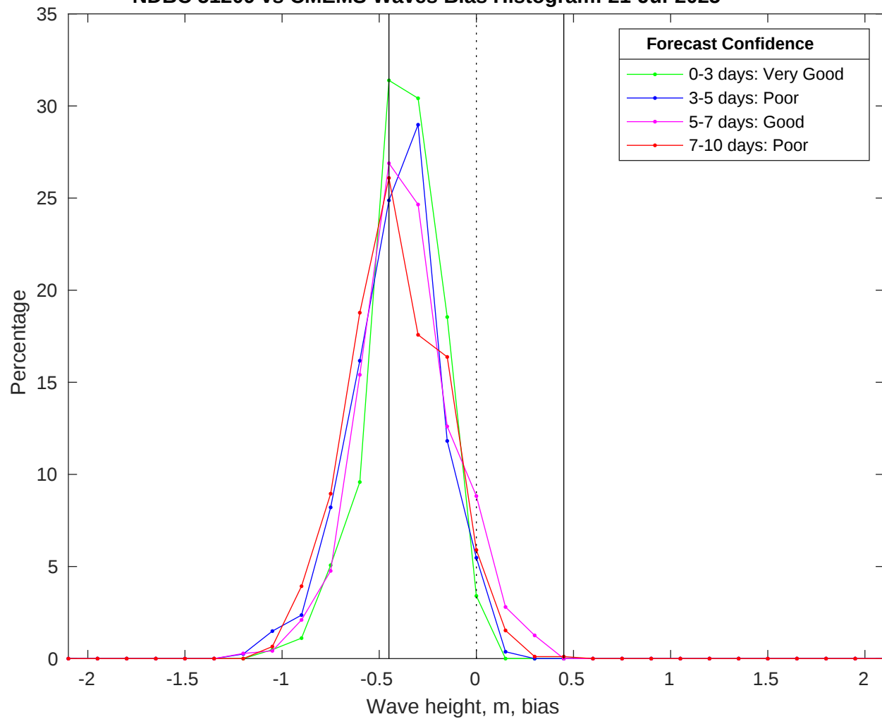
NDBC 51209 vs CMEMS Waves Bias Histogram: 21-Jul-2025
