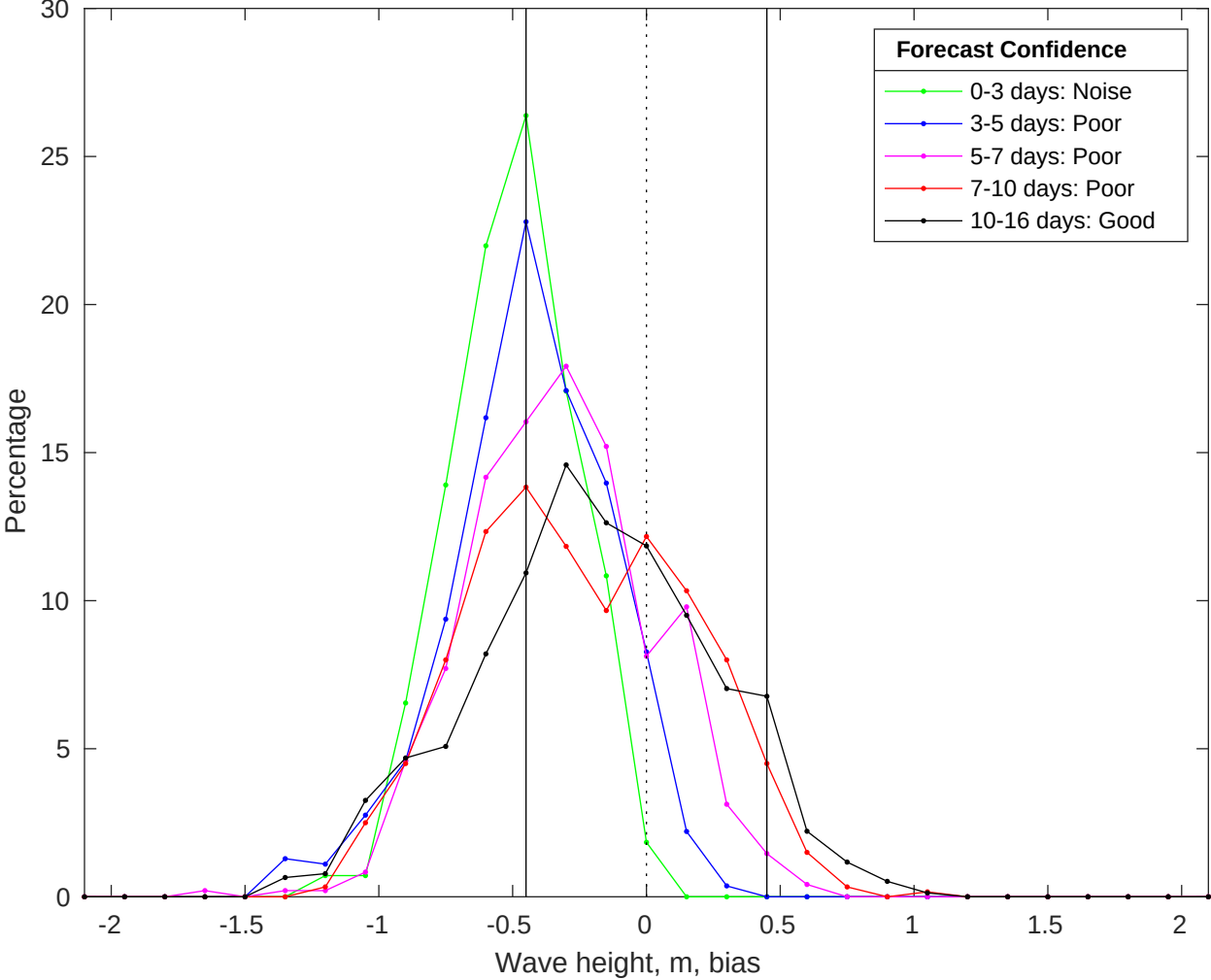
NDBC 51209 vs GFS Waves Bias Histogram: 21-Jul-2025
