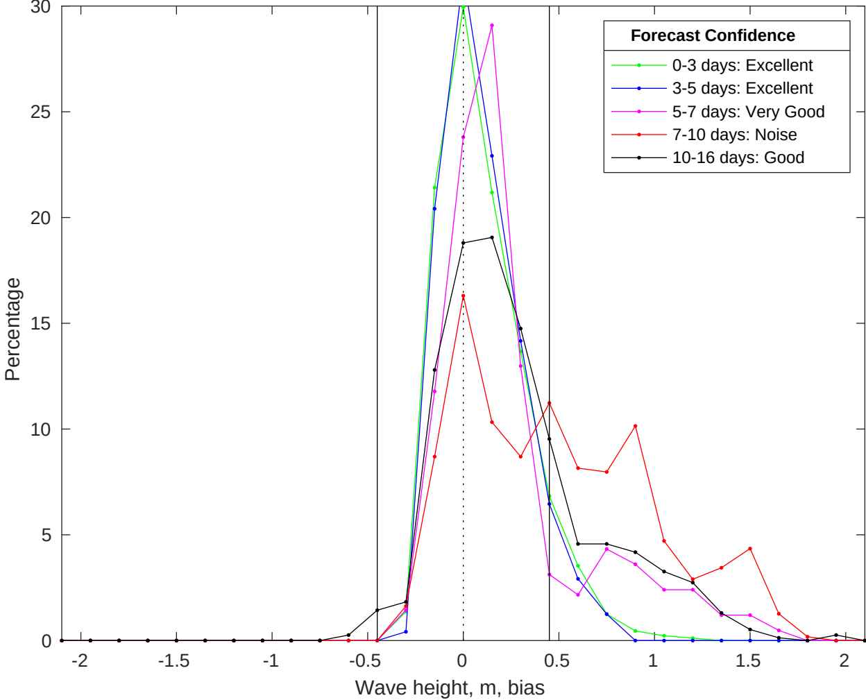
NDBC 52212 vs GFS Waves Bias Histogram: 21-Jul-2025
