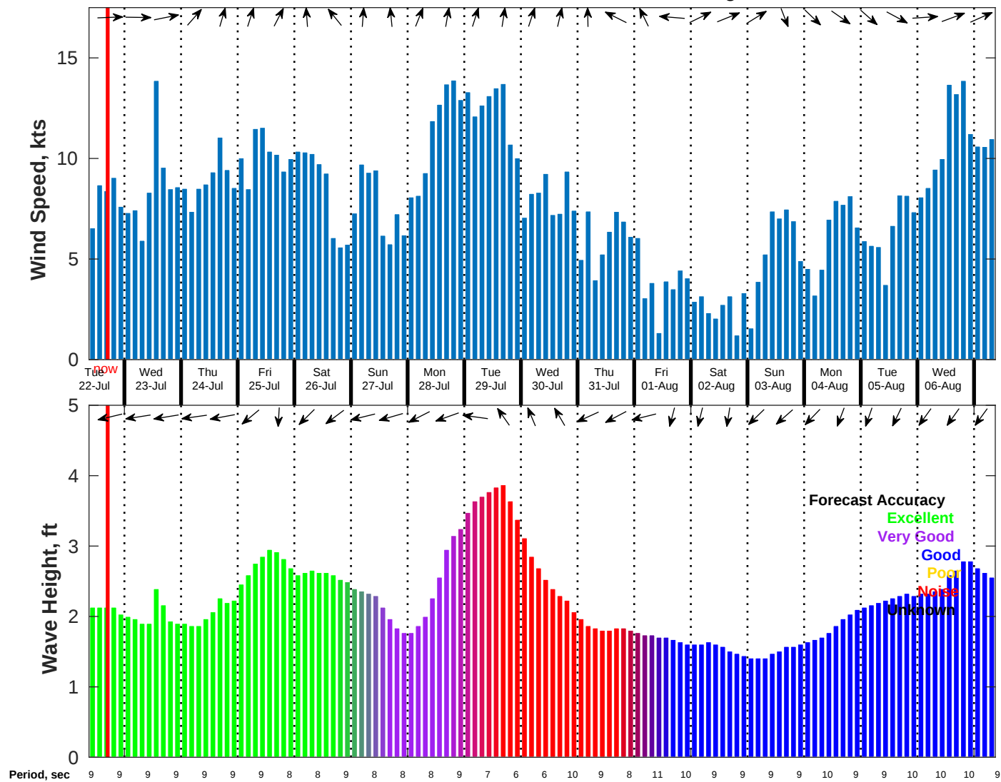
Wind & Wave Forecast for NDBC 52212 from 21-Jul-2025 09:00:00 to 06-Aug-2025 09:00:00
