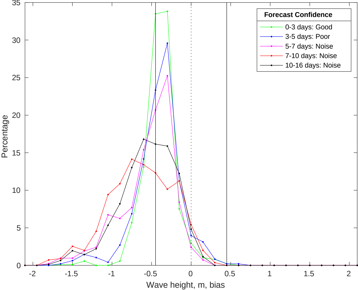
NDBC 52213 vs GFS Waves Bias Histogram: 21-Jul-2025
