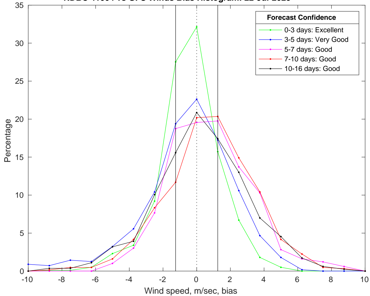
NDBC 41004 vs GFS Winds Bias Histogram: 22-Jul-2025
