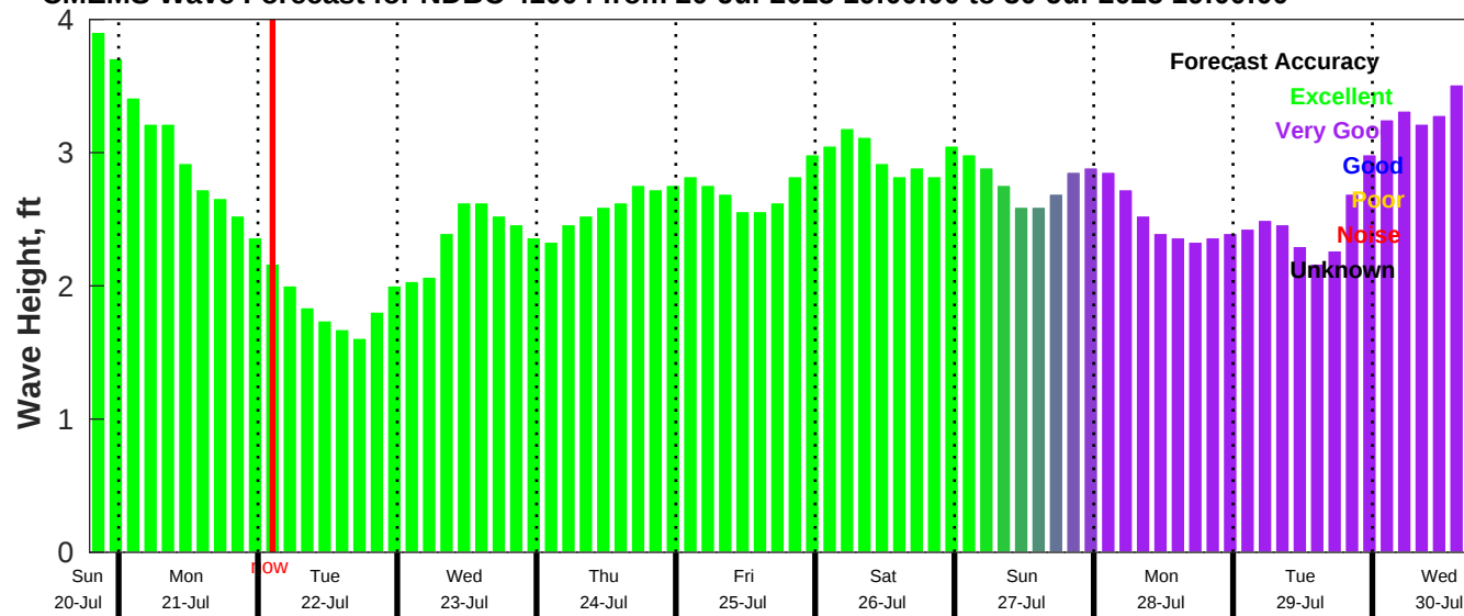
CMEMS Wave Forecast for NDBC 41004 from 20-Jul-2025 19:00:00 to 30-Jul-2025 19:00:00
