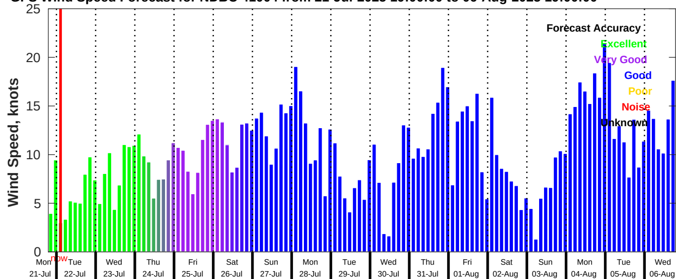
GFS Wind Speed Forecast for NDBC 41004 from 21-Jul-2025 19:00:00 to 06-Aug-2025 19:00:00
