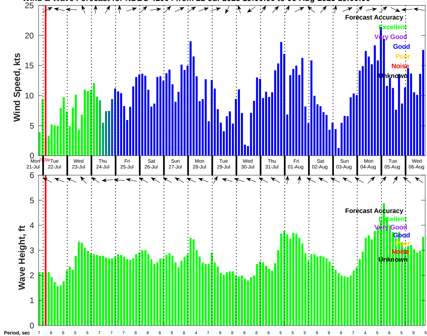
Wind & Wave Forecast for NDBC 41004 from 21-Jul-2025 19:00:00 to 06-Aug-2025 19:00:00
