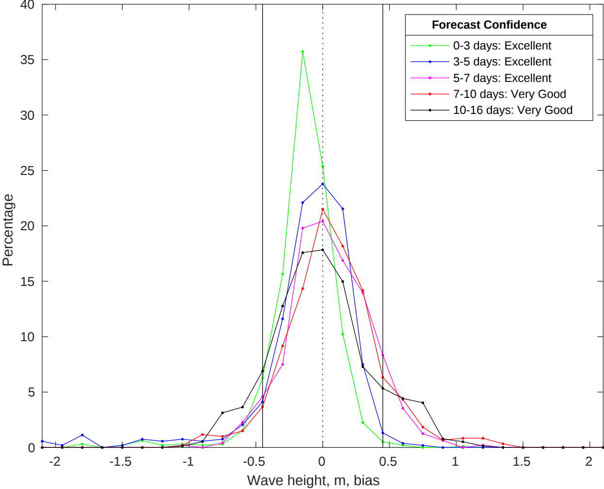
NDBC 41013 vs GFS Waves Bias Histogram: 22-Jul-2025
