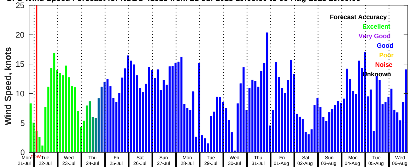
GFS Wind Speed Forecast for NDBC 41013 from 21-Jul-2025 19:00:00 to 06-Aug-2025 19:00:00
