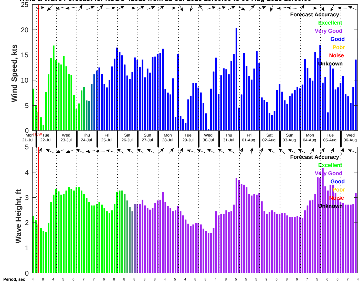
Wind & Wave Forecast for NDBC 41013 from 21-Jul-2025 19:00:00 to 06-Aug-2025 19:00:00
