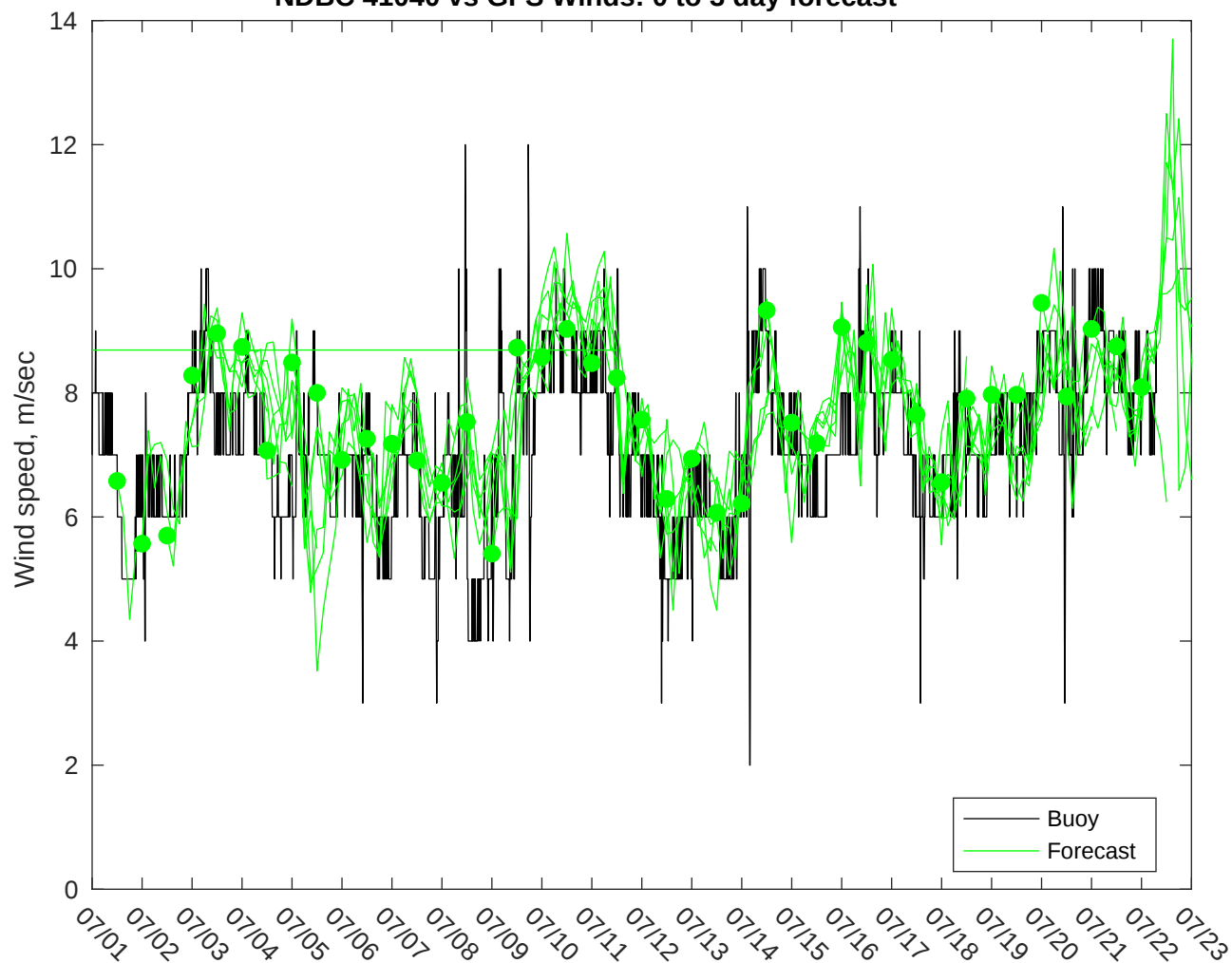
NDBC 41040 vs GFS Winds: 0 to 3 day forecast
