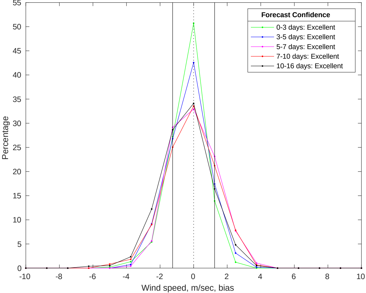
NDBC 41040 vs GFS Winds Bias Histogram: 22-Jul-2025
