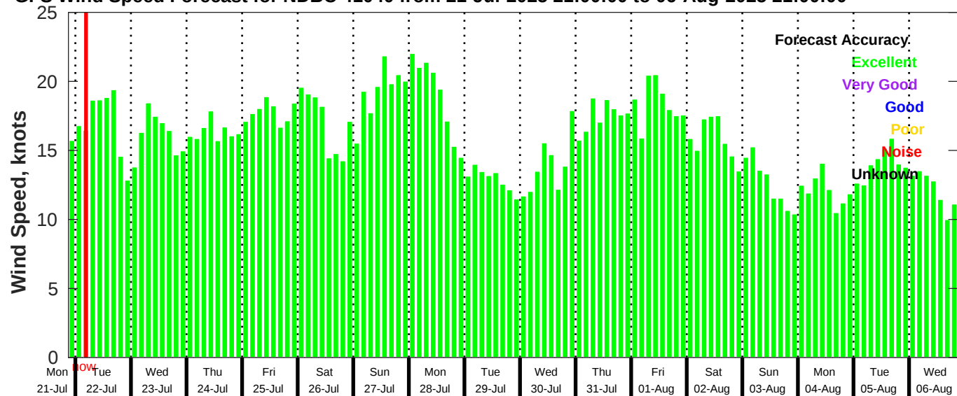
GFS Wind Speed Forecast for NDBC 41040 from 21-Jul-2025 21:00:00 to 06-Aug-2025 21:00:00
