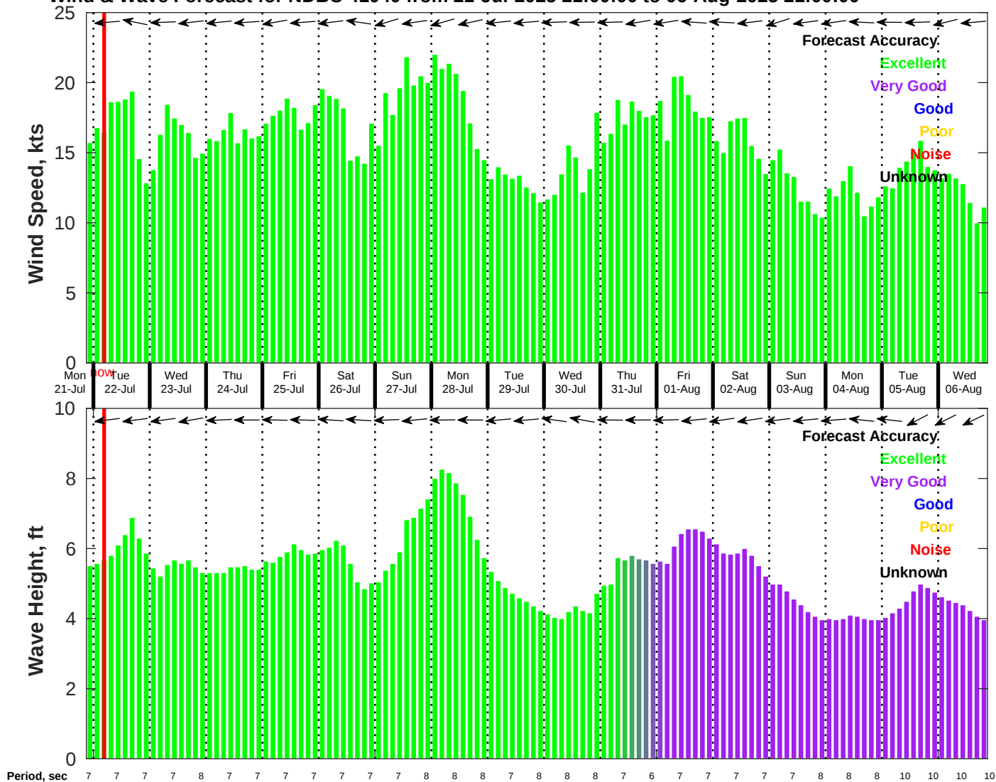
Wind & Wave Forecast for NDBC 41040 from 21-Jul-2025 21:00:00 to 06-Aug-2025 21:00:00
