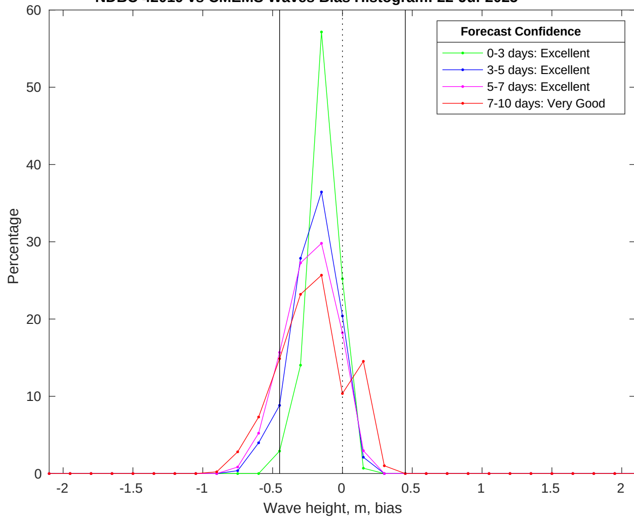
NDBC 42019 vs CMEMS Waves Bias Histogram: 22-Jul-2025
