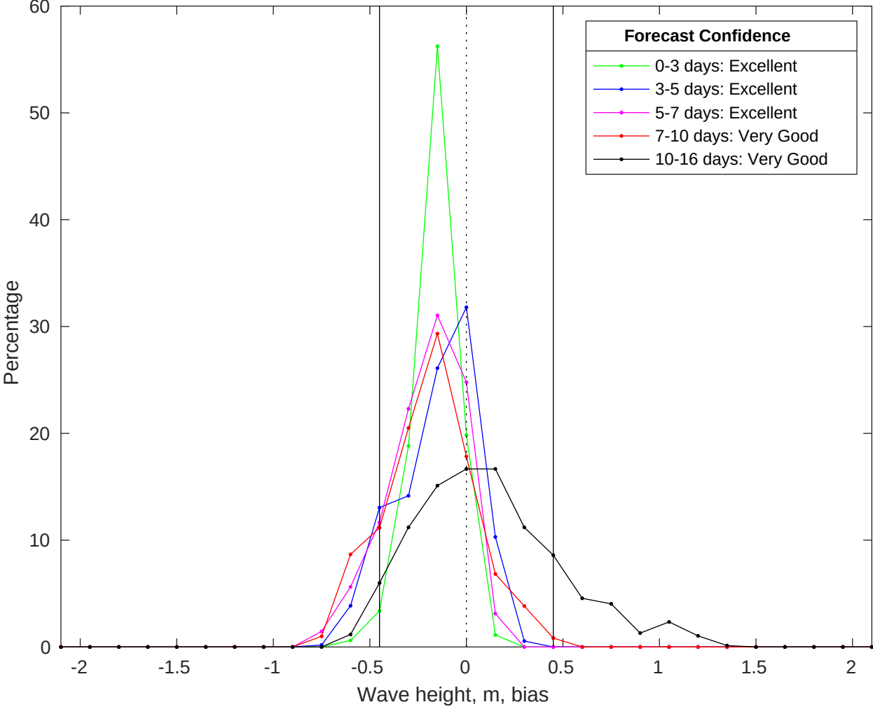
NDBC 42019 vs GFS Waves Bias Histogram: 22-Jul-2025
