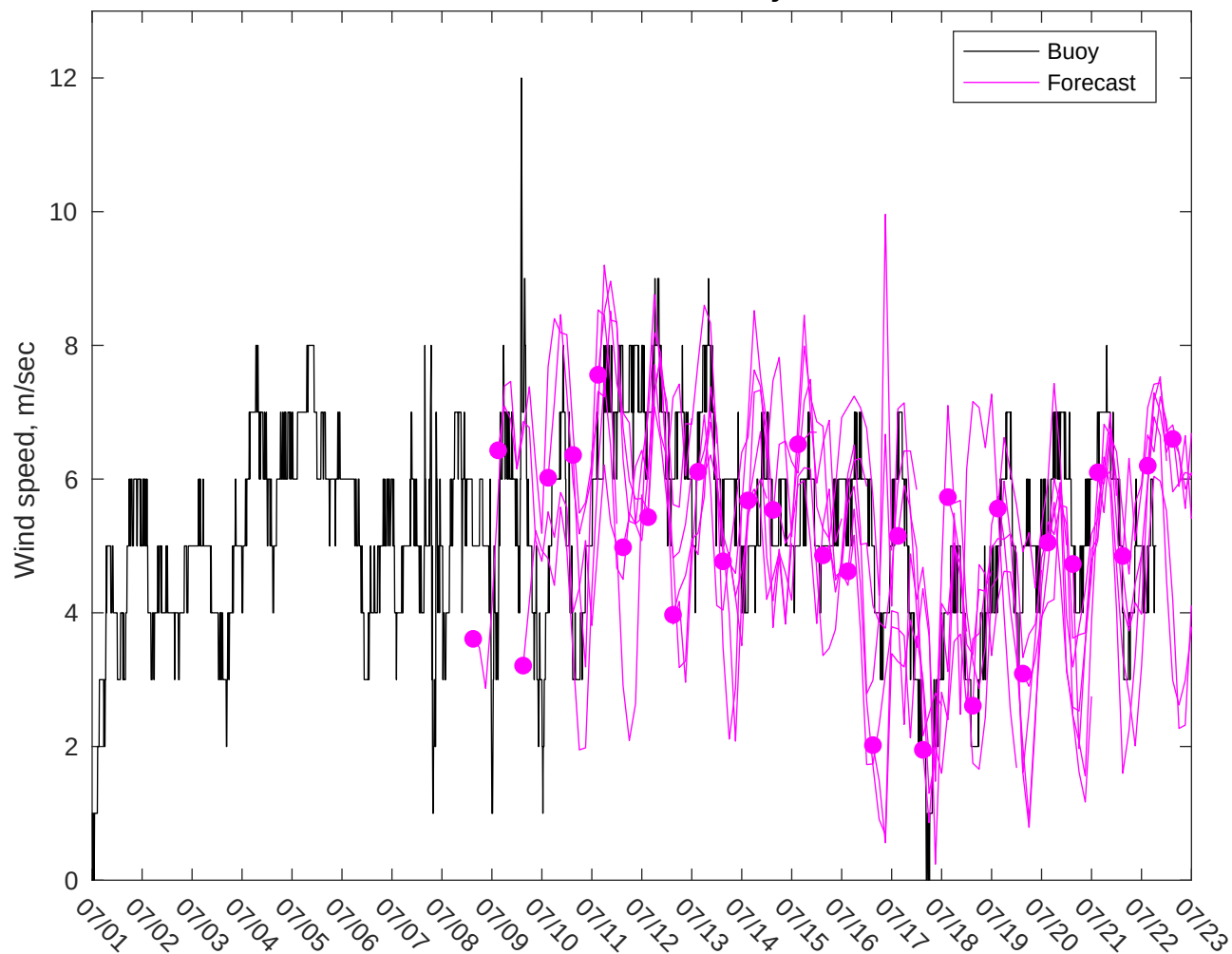
NDBC 42019 vs GFS Winds: 7 to 10 day forecast
