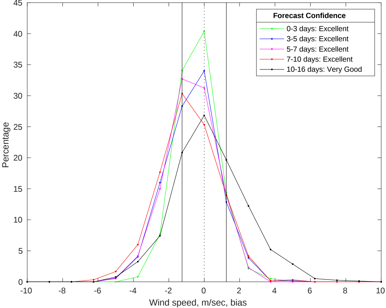
NDBC 42019 vs GFS Winds Bias Histogram: 22-Jul-2025
