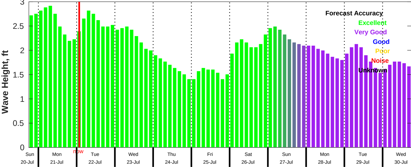
CMEMS Wave Forecast for NDBC 42019 from 20-Jul-2025 18:00:00 to 30-Jul-2025 18:00:00
