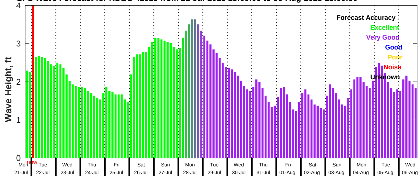
GFS Wave Forecast for NDBC 42019 from 21-Jul-2025 18:00:00 to 06-Aug-2025 18:00:00
