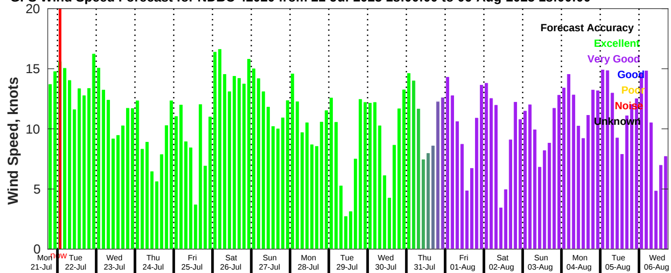
GFS Wind Speed Forecast for NDBC 42020 from 21-Jul-2025 18:00:00 to 06-Aug-2025 18:00:00
