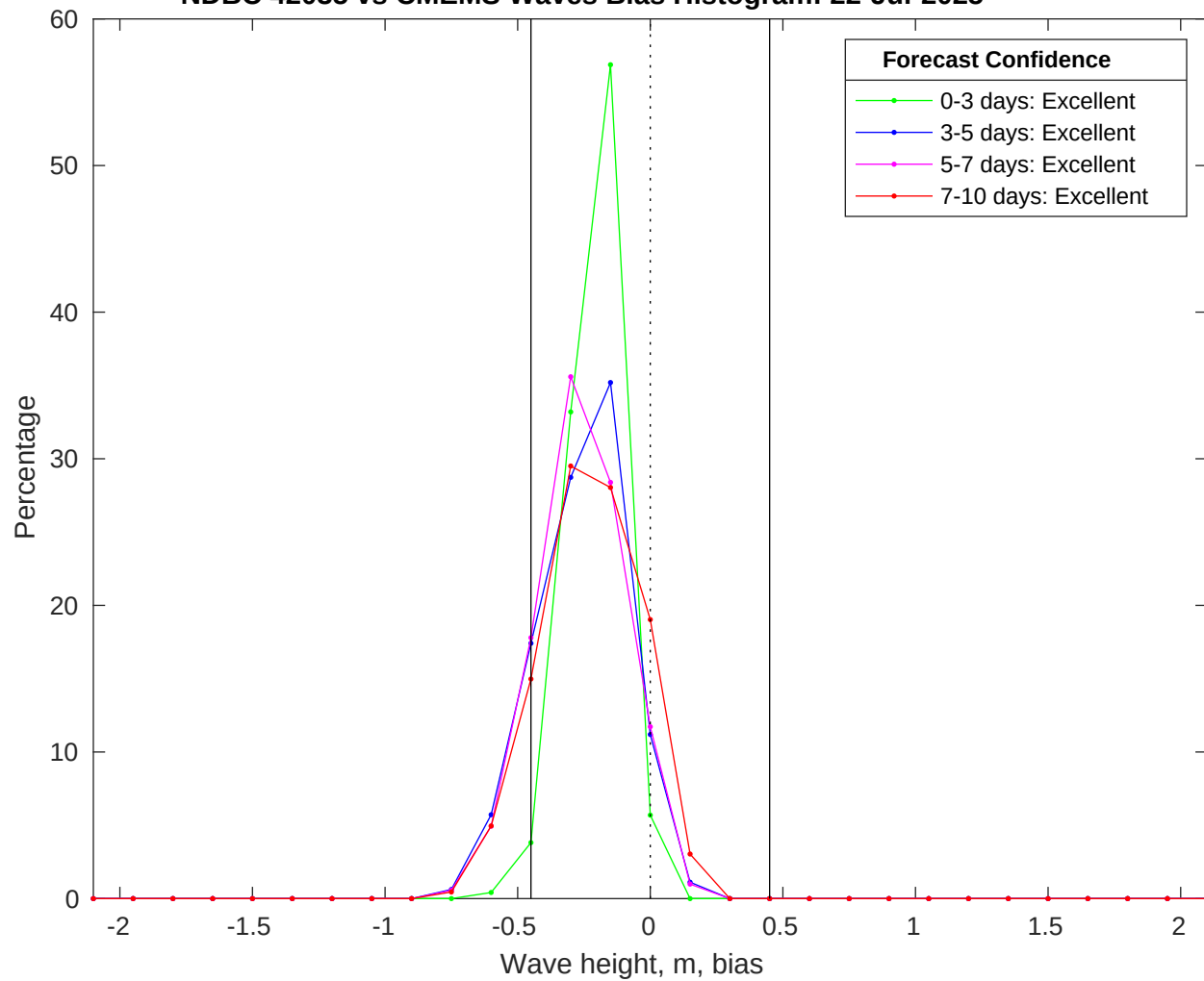
NDBC 42035 vs CMEMS Waves Bias Histogram: 22-Jul-2025
