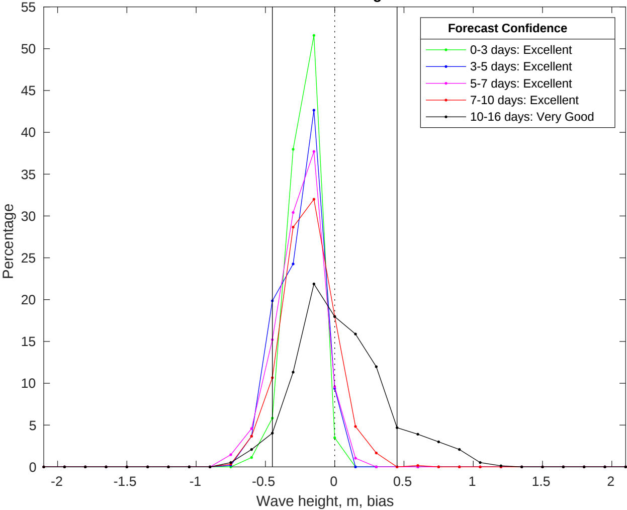
NDBC 42035 vs GFS Waves Bias Histogram: 22-Jul-2025
