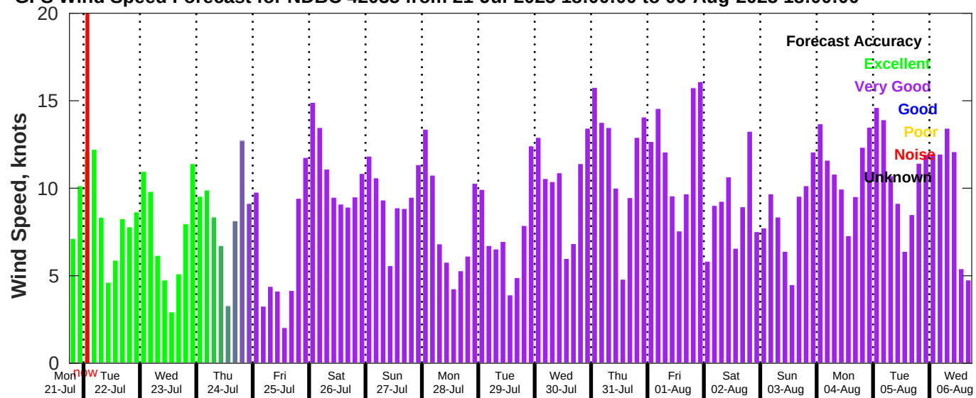
GFS Wind Speed Forecast for NDBC 42035 from 21-Jul-2025 18:00:00 to 06-Aug-2025 18:00:00
