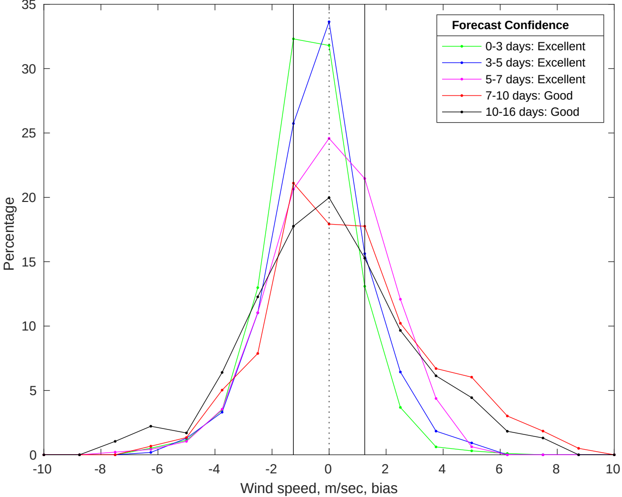
NDBC 42036 vs GFS Winds Bias Histogram: 22-Jul-2025
