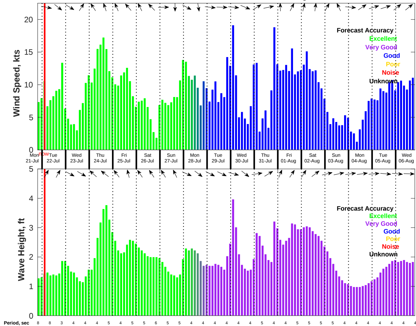
Wind & Wave Forecast for NDBC 42036 from 21-Jul-2025 19:00:00 to 06-Aug-2025 19:00:00
