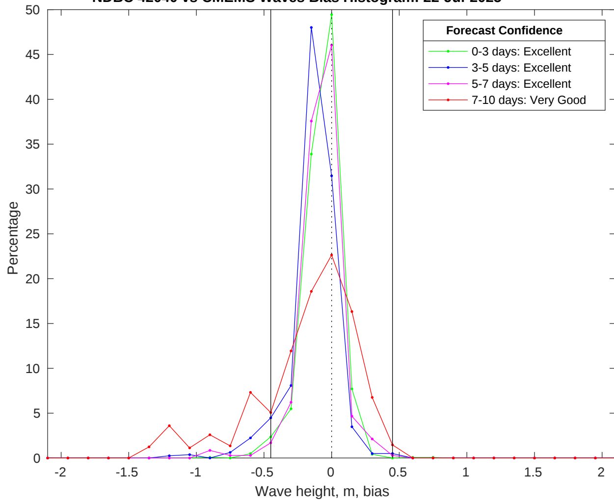
NDBC 42040 vs CMEMS Waves Bias Histogram: 22-Jul-2025
