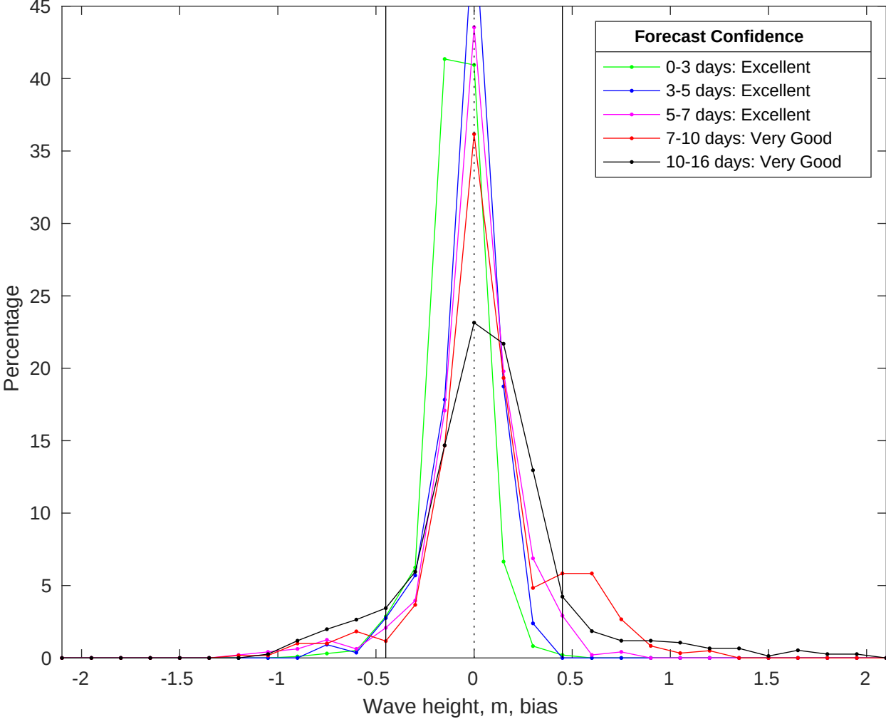
NDBC 42040 vs GFS Waves Bias Histogram: 22-Jul-2025
