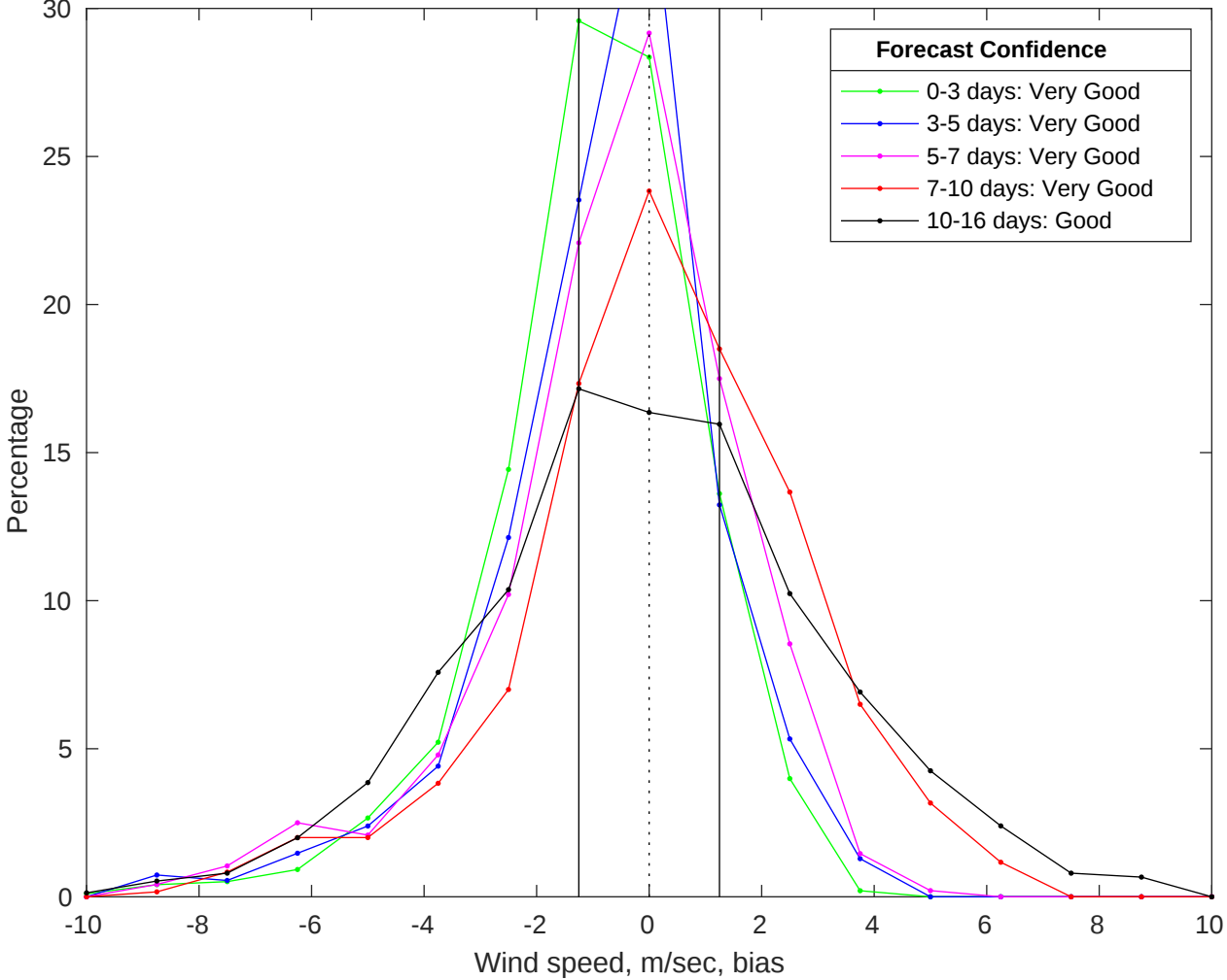
NDBC 42040 vs GFS Winds Bias Histogram: 22-Jul-2025
