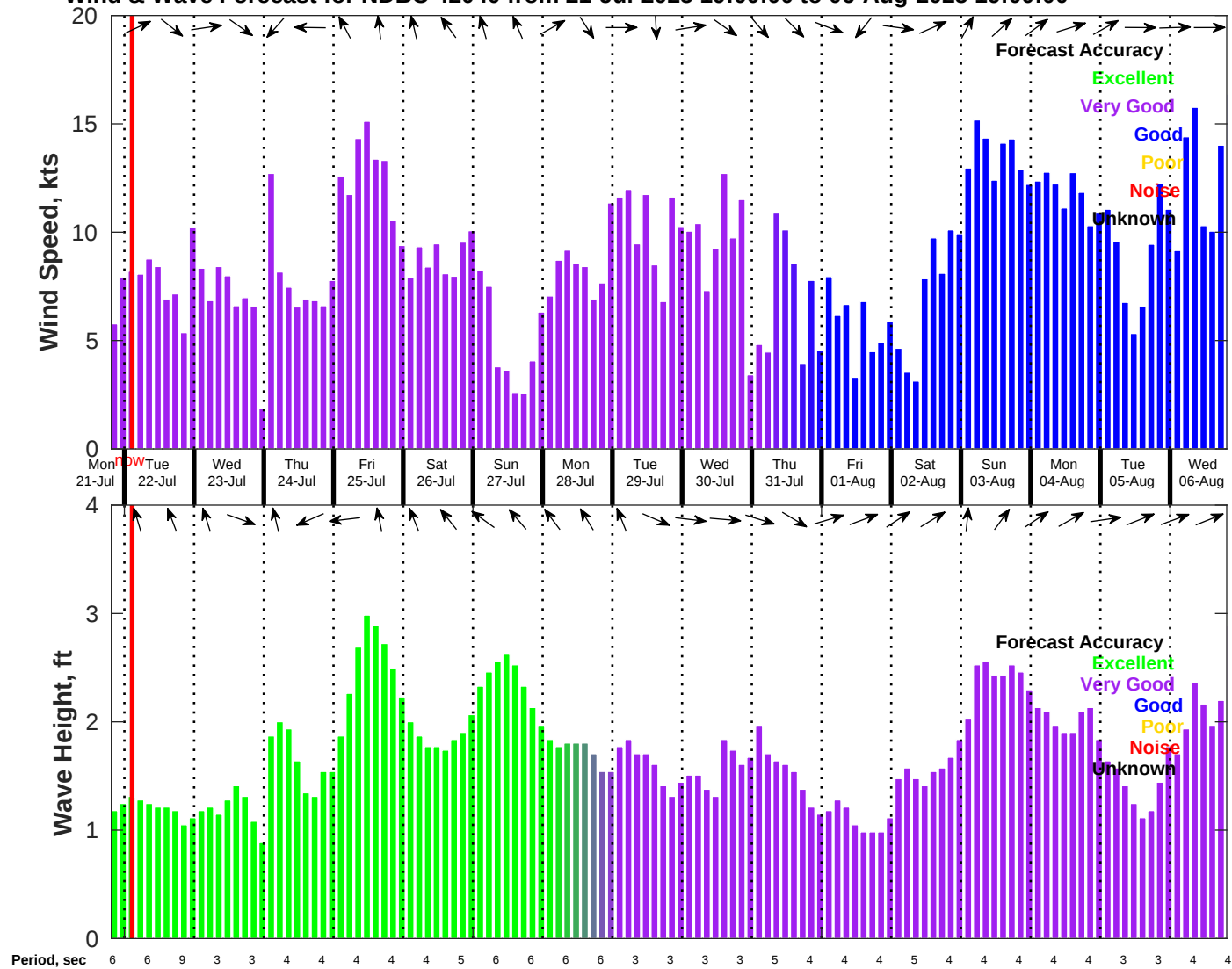
Wind & Wave Forecast for NDBC 42040 from 21-Jul-2025 19:00:00 to 06-Aug-2025 19:00:00
