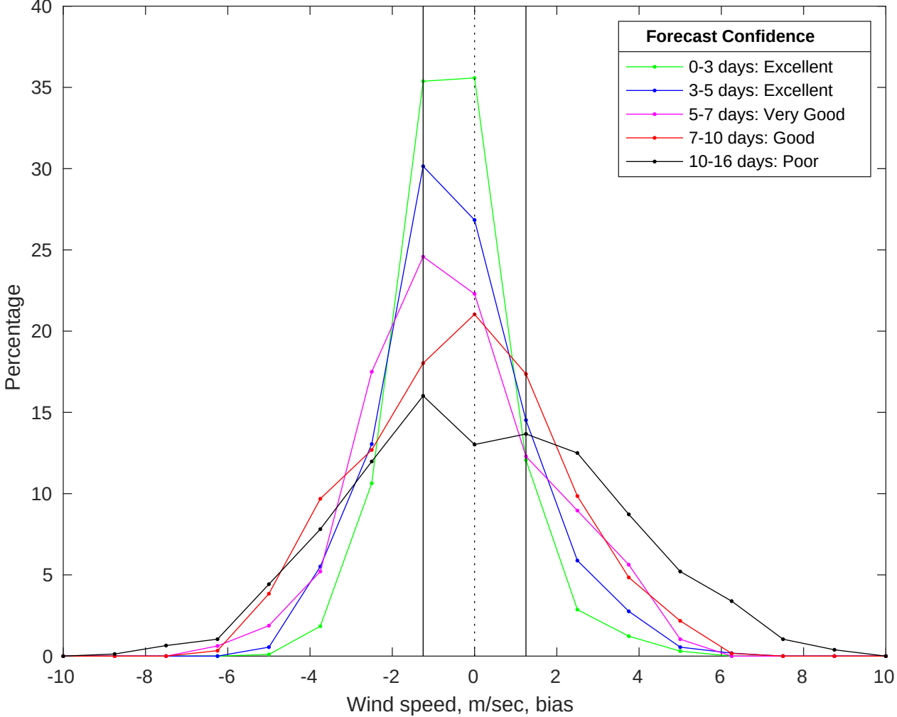
NDBC 46011 vs GFS Winds Bias Histogram: 22-Jul-2025
