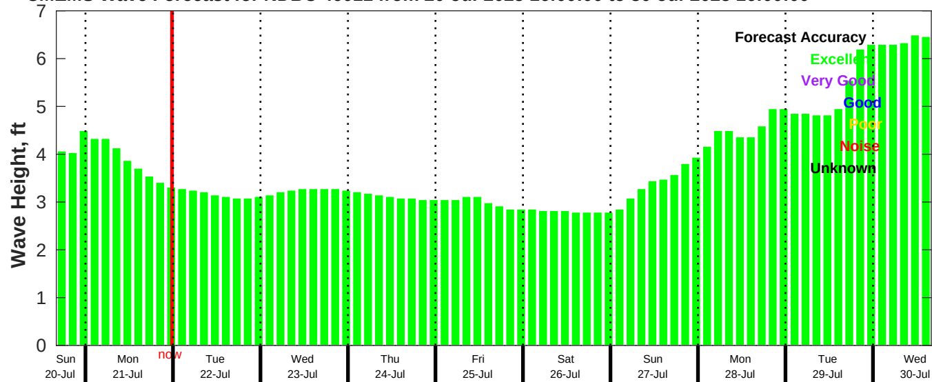
CMEMS Wave Forecast for NDBC 46011 from 20-Jul-2025 16:00:00 to 30-Jul-2025 16:00:00
