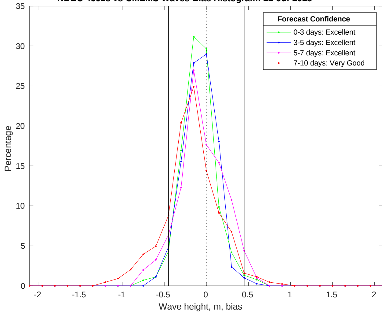
NDBC 46028 vs CMEMS Waves Bias Histogram: 22-Jul-2025
