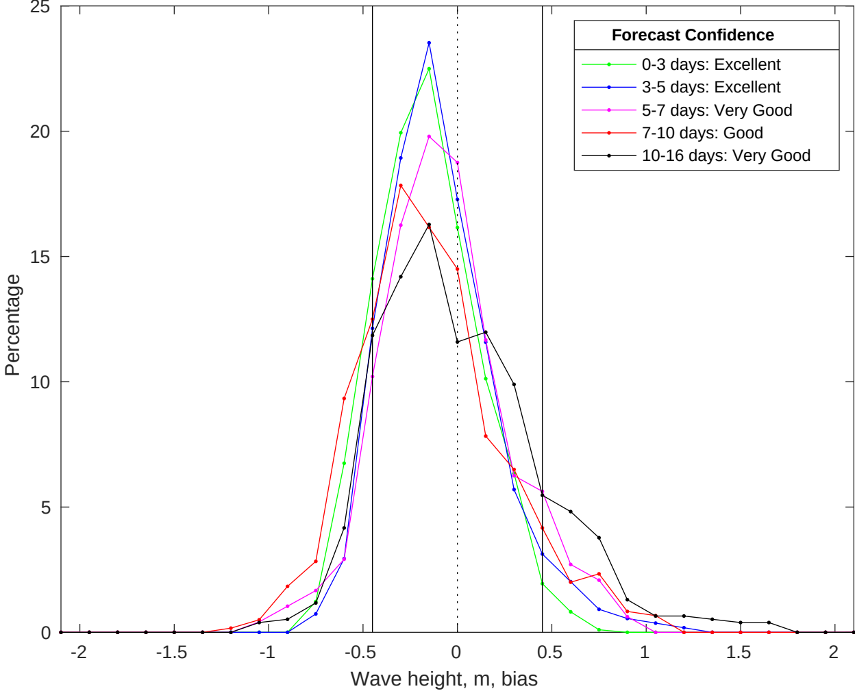
NDBC 46028 vs GFS Waves Bias Histogram: 22-Jul-2025
