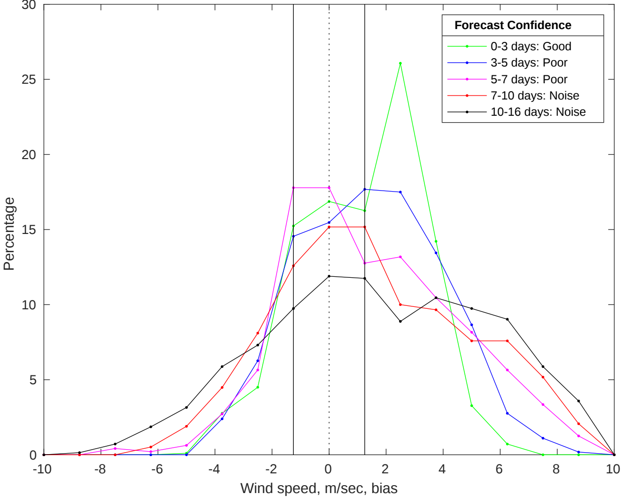
NDBC 46028 vs GFS Winds Bias Histogram: 22-Jul-2025
